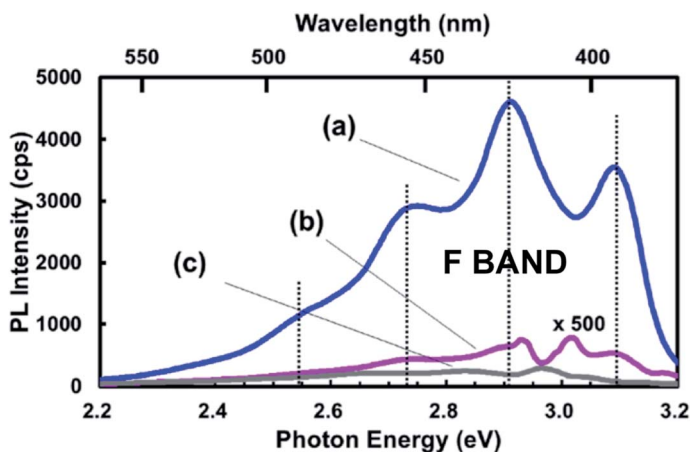
Fig. 16 Photoluminescence of adsorbed fluorescent organic contaminants on silicon nanoparticles. 268 Adapted with permission from T. Matsumoto, M. Maeda and H. Kobayashi, Nanoscale Res. Lett. , 2016, 11(7), available via an open access CC-BY license.
