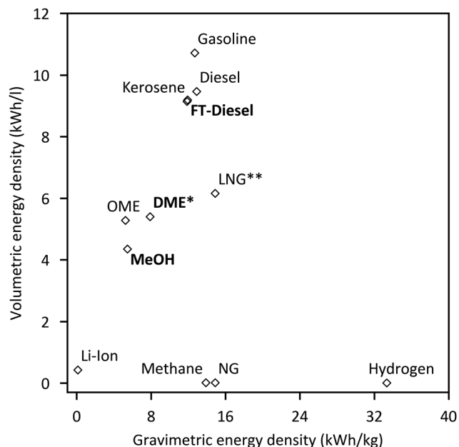
Fig. 1 Gravimetric and volumetric energy density of different fuels and Li-Ion batteries for comparison (*at 10 bar; **at -160\text{ }^{\circ}\text{C} ). 13–15
