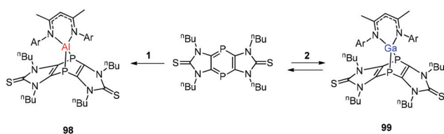
Scheme 24 Reaction of tricyclic 1,4-diphosphinine with \text{DippNacAl}(\text{i}) ( 1 ) and \text{DippNacGa}(\text{i}) ( 2 ) to get 7-metalla-1,4-diphosphanorbornadienes 98 and 99 .
