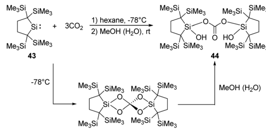
Scheme 20 Synthesis of the bis(silyl)carbonate 44 by the reaction of dialkylsilylene 43 with \text{CO}_2 .
