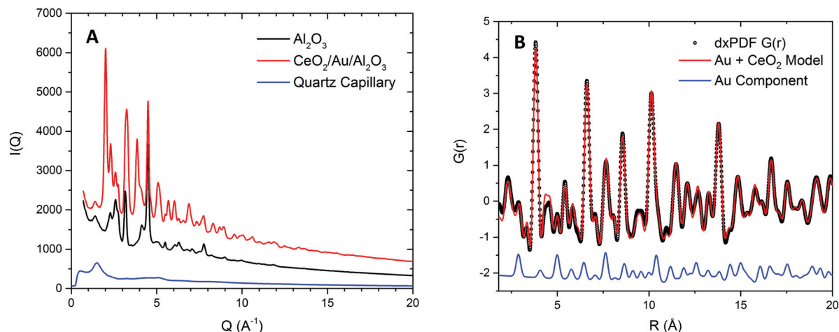
Fig. 2 Experimental DPDF patterns, alumina subtraction and Fourier Transformation recorded at room temperature. (A) Integrated total scattering pattern relating to: a ceria alumina support Au inverse catalyst sample, a gamma alumina support and fused quartz capillary sample environment; illustrating the process for correction to arrive at the differential xPDF containing the fluorite ceria and metallic Au components. (B) Example fit to the initial differential xPDF G(r) for a biphasic model containing fluorite ceria and metallic Au components over a fitting region of 1.8 to 20 Å. The metallic Au component contribution is highlighted below the data to illustrate the presence of the metallic Au phase within the extracted differential xPDF G(r) . Typical fit residual, r_w = 0.1 .
