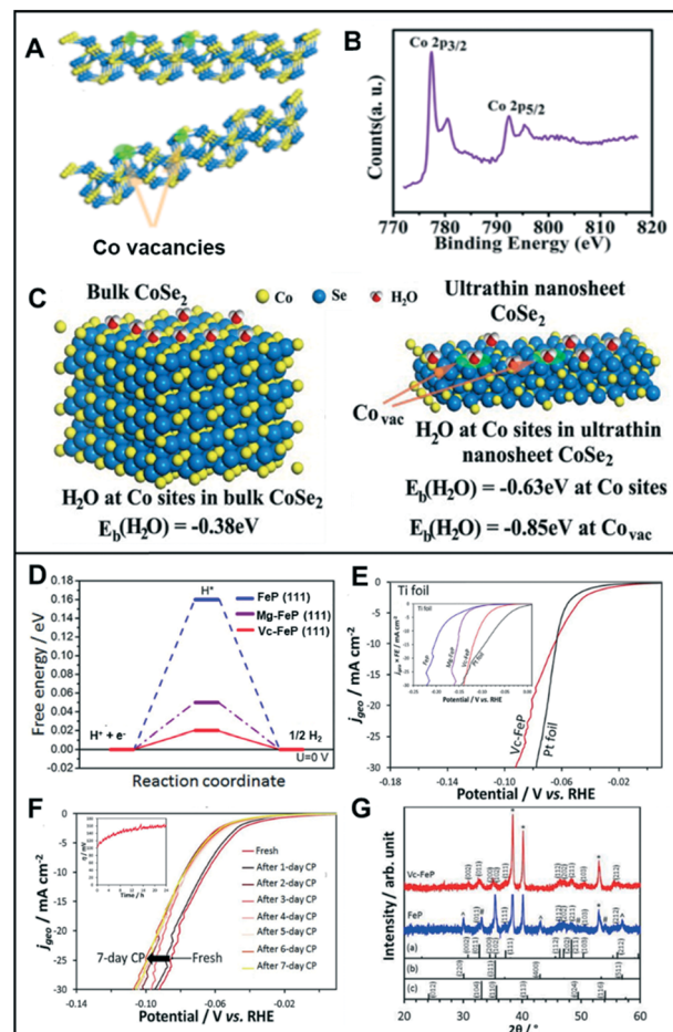
Fig. 6 (A) Schematic illustration of the formation of Co vacancies in \text{CoSe}_2 ultrathin nanosheets. (B) The XPS Co 2p of \text{CoSe}_2 ultrathin nanosheets. (C) Geometries and binding energies of \text{H}_2\text{O} molecules on Co sites and vacancies for bulk \text{CoSe}_2 (left) and ultrathin nanosheet \text{CoSe}_2 (right). Reproduced with permission from ref. 36. Copyright 2014 American Chemical Society. (D) Free energy diagram of FeP, Mg-FeP, and Vc-FeP (111) surfaces. (E) Polarization curves for the HER activity of Vc-FeP in 0.5 M \text{H}_2\text{SO}_4 (inset: HER activity in 1 M KOH). (F) The CP tests of Vc-FeP in 0.5 M \text{H}_2\text{SO}_4 (inset: stability test on Vc-FeP performed in 1 M KOH). (G) XRD data for FeP and Vc-FeP. The reference patterns of (a) orthorhombic FeP, (b) \gamma\text{-Fe}_2\text{O}_3 , and (c) \alpha\text{-Fe}_2\text{O}_3 also are shown. Reproduced with permission from ref. 37. Copyright 2017 Wiley-VCH.
