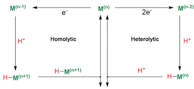
Fig. 9 Proposed mechanistic pathways for \text{H}_2 evolution by a metallic catalytic center.
