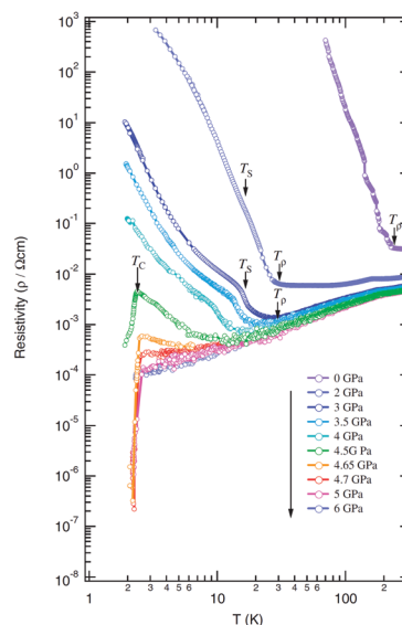
Fig. 16 Temperature dependence of resistivity of (\text{TMTTF})_2\text{AsF}_6 under various pressures, where T_m , T_s , and T_c are temperatures at minimum resistivity, spin-Peierls transition, and superconducting transition, respectively. Adapted with permission from ref. 72. Copyright 2007 Physical Society of Japan.
