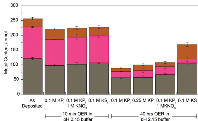
Fig. 4 Total metal content, Pb (grey), Fe (brown), and Co (magenta) of 1 \text{ cm}^2 CoFePbO x films after operation in specified buffers at pH 2.15 for 0 min, 10 min, or 40 h at 1 \text{ mA cm}^{-2} for OER.
