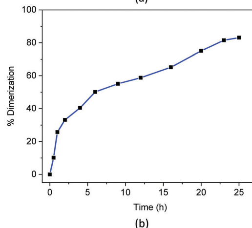
Fig. 2 (a) ^1\text{H-NMR} spectra of 1 (30 min grinding) in \text{DMSO-}d_6 plotted at different times of UV irradiation. Complete absence of the \text{H}_a , \text{H}_b protons may indicate quantitative consumption of the 5-Spym ligand. However, some unidentified peaks indicate only 83% of rcctt -bpceb photoproduct formed. (b) Time-dimerization plot for 30 min ground sample shows the progress of the photoreaction under UV light with time.
