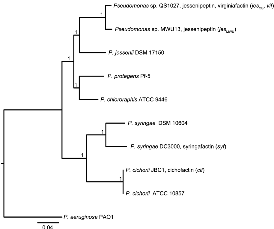
Fig. 6 Top: Molecular phylogeny of the lipopeptide-producing Pseudomonas species based on multilocus sequence typing (MLST) of 16S rRNA genes and five housekeeping genes ( gyrB , nuoCD , lfeS , ppsA , rpoB ). The tree was inferred by Maximum Likelihood estimation using a concatenated alignment as input. The P. aeruginosa PAO1 sequence was used as an outgroup to root the tree. The scale bar indicates substitutions per site.
