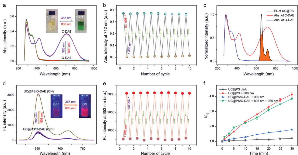
Fig. 2 (a) UV-vis-NIR absorption spectra and (b) absorption intensity changes at 712 nm of the photochromic DAE upon alternating UV (365 nm, 5\text{ mW cm}^{-2} , 1 min) and NIR (808 nm, 0.25\text{ W cm}^{-2} , 30 s) light irradiation. The inset in (a) shows the changes of its photographic image. (c) UV-vis-NIR absorption (Abs.) spectra of two different forms of DAE and the fluorescence spectrum of UC@PS. The overlapping of spectra is indicated in orange. (d) Fluorescence spectra and (e) fluorescence intensity changes at \lambda_{\text{max}} = 653\text{ nm} of UC@PS/C-DAE upon alternating UV (365 nm, 5\text{ mW cm}^{-2} , 1 min) and NIR (808 nm, 0.25\text{ W cm}^{-2} , 30 s) light irradiation ( \lambda_{\text{ex}} = 420\text{ nm} ). The inset in (e) shows the changes of its photographic fluorescence image. (f) Singlet oxygen generation by UC@PS and UC@PS/DAE upon irradiation with light of different wavelengths in water (808 nm, 0.25\text{ W cm}^{-2} , and 980 nm, 1.2\text{ W cm}^{-2} ), detected by SOSG assay. Data are means \pm SD; N = 3 .
