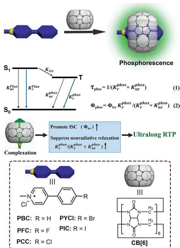
Scheme 1 Schematic illustration of the solid-state supramolecular strategy and Jablonski diagram for radiative and non-radiative processes. ( K_r^{\text{fluor}} is the radiative rate constant of the lowest excited singlet state S_1 ; K_{\text{nr}}^{\text{fluor}} is the nonradiative rate constant of the lowest excited singlet state S_1 ; K_{\text{isc}} is the intersystem crossing rate constant from the excited singlet state to the triplet state; K_r^{\text{phos}} is the radiative rate constant of the lowest excited triplet state T_1 ; K_{\text{nr}}^{\text{phos}} is the nonradiative rate constant of the lowest excited triplet state T_1 ; \tau_{\text{phos}} is the lifetime of the excited triplet state; \Phi_{\text{phos}} is the quantum yield of phosphorescence; and \Phi_{\text{isc}} is the quantum yield of intersystem crossing from the excited singlet state to the triplet state; inset: the molecular structures of the guests and host).
