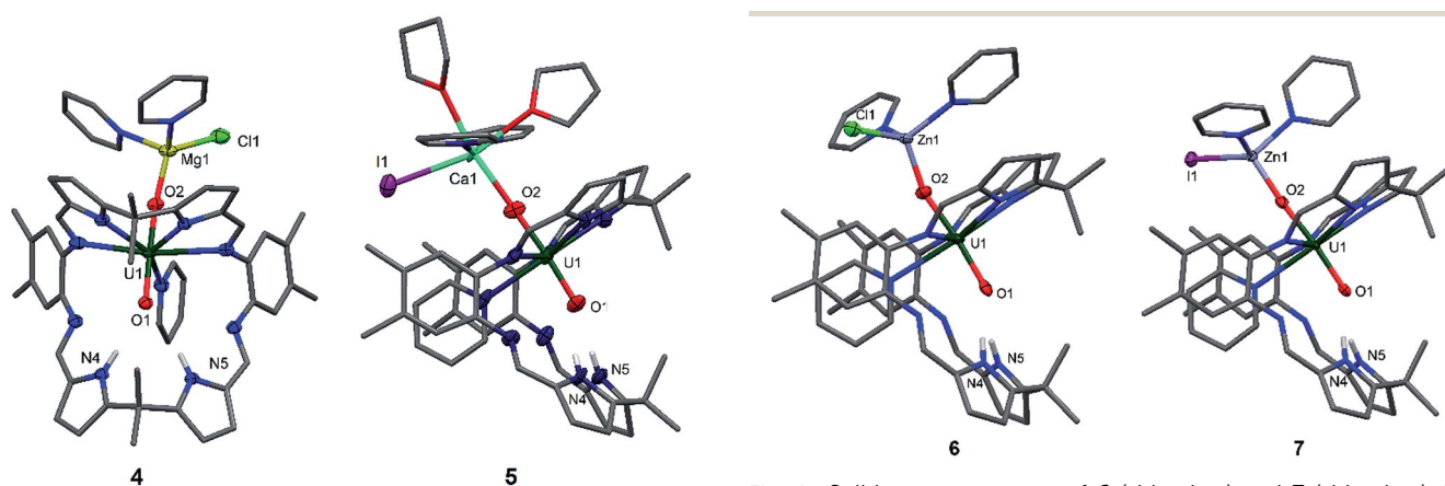
Fig. 3 Solid-state structures of 4 (front view) and 5 (side view). For clarity, all hydrogen atoms except the pyrrole N–Hs and all solvent molecules are omitted (displacement ellipsoids are drawn at 50% probability). Selected bond lengths (Å) for 4 : U1–O1 1.864(2), U1–O2 1.909(2), O1–N4 2.889(3), O1–N5 3.040(3). O1–U1–O2 bond angle: 174.21(9)°. Selected bond lengths for 5 : U1–O1 1.88(1), U1–O2 1.90(1), Ca1–O2 2.33(1), O1–N4 2.95(2), O1–N5 2.92(2). O1–U1–O2 bond angle: 176.0(6)°.
