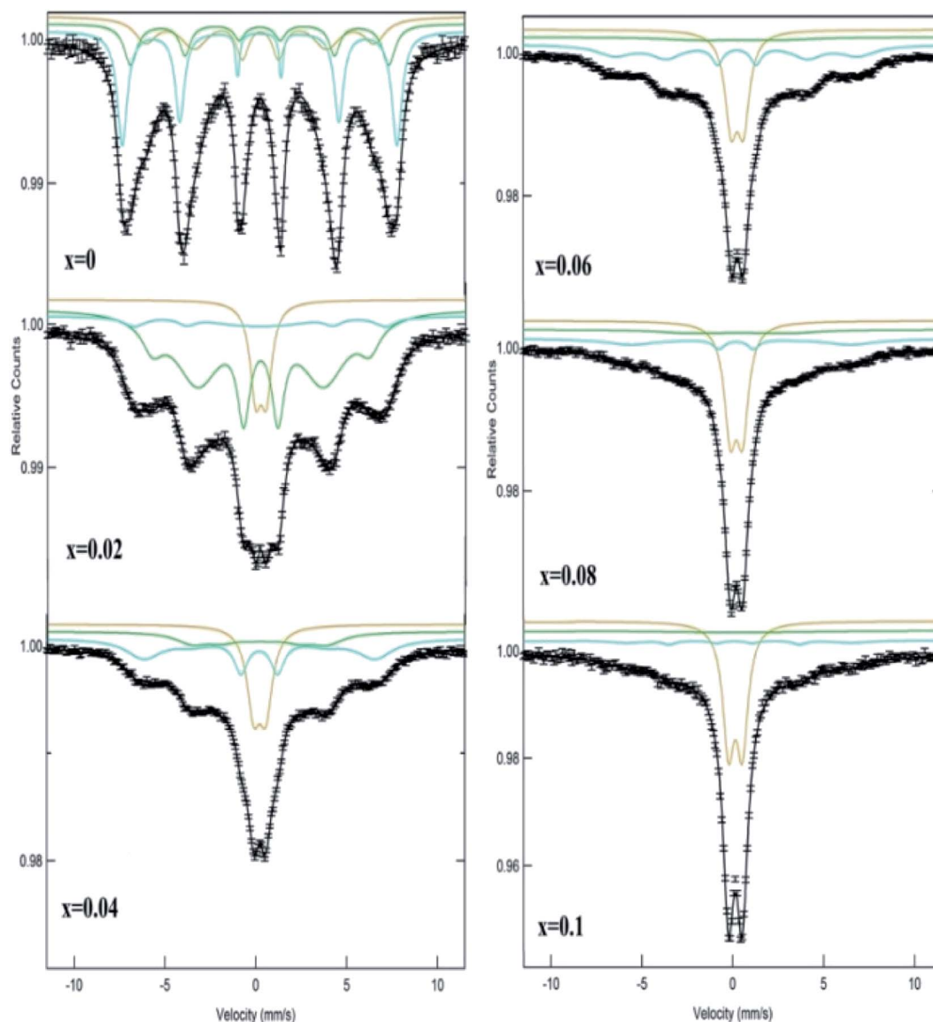
Fig. 7 RT Mössbauer spectra of \text{Ni}_{0.4}\text{Cu}_{0.2}\text{Zn}_{0.4}\text{La}_x\text{Y}_x\text{Fe}_{2-x}\text{O}_4 ( x = 0.00 - 0.10 ) NSF.
