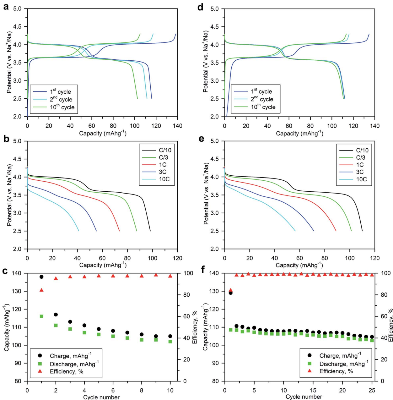
Fig. 7 Electrochemical performance of Na 3 V 2 O 2 (PO 4 ) 2 F (a–c) annealed with glucose (8 wt%) at 600 °C for 1 h, and (d–f) coated with dopamine for 24 h and annealed at 500 °C for 3 h, over the potential range 2.5–4.3 V vs. Na + /Na at room temperature: (a and d) galvanostatic charge–discharge profiles at a C/10 current density; (b and e) galvanostatic discharge profiles at different current densities; (c and f) capacity retention and coulombic efficiency at a C/10 current density.
