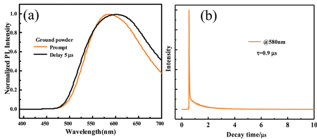
Fig. 7 (a) Prompt and delayed (5 \mu s) photoluminescence spectra of the ground powder of ODFRPTZ. (b) The decay curve of the delayed fluorescence.
