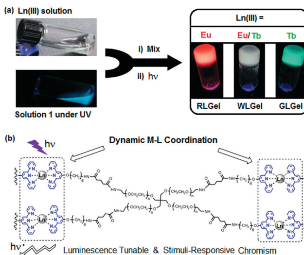
Fig. 4 (a) Schematic preparation of Ln(III) coordination-based luminescent metallo gels under UV light; (b) chemical structure of terpy-end-capped 4-arm PEG polymer cross-linked via Ln-terpy coordination. 50
