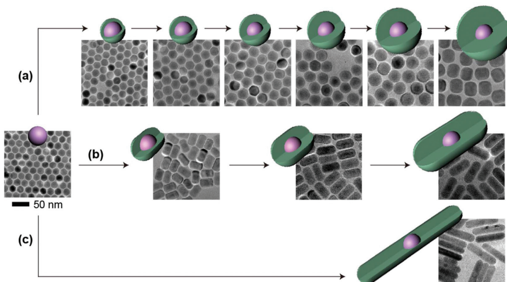
Fig. 5 Schematic presentation and TEM images showing the isotropic and anisotropic growth of the \text{NaYF}_4 inert shell on 0.2 \text{ mmol mL}^{-1} \text{NaYF}_4:\text{Yb}/\text{Er}(20/2\%) upconversion nanoparticles. (a) Isotropic shell growth via a layer-by-layer method with the addition of 0.2 \text{ mmol} of shell precursors in each step. (b) Anisotropic shell growth via a layer-by-layer method with the addition of 0.4 \text{ mmol} of shell precursors in each step. (c) Anisotropic shell growth on \text{NaYF}_4:\text{Yb}/\text{Er}(20/2\%) core with the addition of 1.2 \text{ mmol} of shell precursors.
