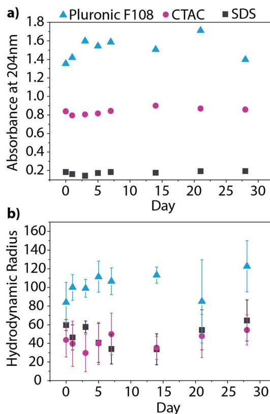
Fig. 7 BNNT dispersions in SDS, CTAC, and Pluronic F108 tracked over one month by (a) UV absorbance and (b) DLS. Both measurements show no significant changes over time confirming that the dispersions are stable.
