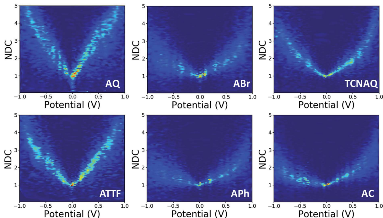
Fig. 5 Normalized differential conductance heatmaps for \text{Au}^{\text{Mica}}/\text{SAM}/\text{EGaIn} junctions comprising AQ, ABr, TCNAQ, ATTF, APh, and AC.
