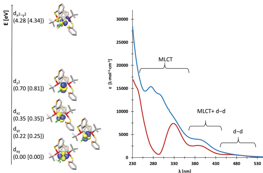
Fig. 3 Left: Orbital scheme for the d orbitals in 1 and 2 (energies for 2 are given in brackets). Exemplarily, the d orbitals for 1 are shown with an isosurface value of 0.05. Right: UV-vis spectra of 1 (blue) and 2 (red) in diethyl ether.
