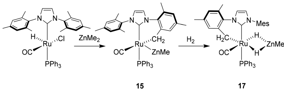
Scheme 6 Formation of [Ru(\text{IMes})(\text{PPh}_3)(\text{CO})\text{ZnMe}] ( 15 ) and [Ru(\text{IMes})(\text{PPh}_3)(\text{CO})(\text{H})_2\text{ZnMe}] ( 17 ).
