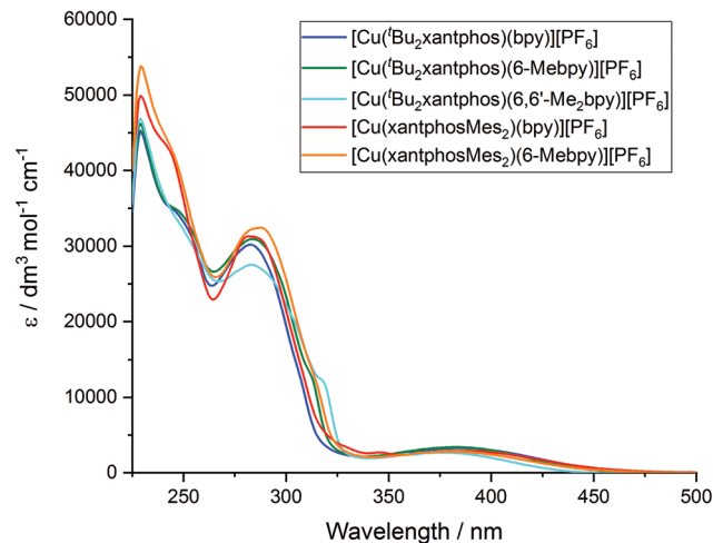
Fig. 11 Solution absorption spectra of [\text{Cu}(\text{P}^{\wedge}\text{P})(\text{N}^{\wedge}\text{N})][\text{PF}_6] complexes (CH 2 Cl 2 , 2.5 \times 10^{-5} mol dm -3 ).
