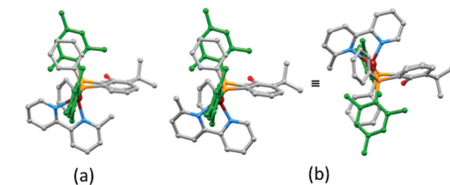
Fig. 5 Upper: Proposed dynamic processes in [\text{Cu}(\text{xantphos})(\text{bpy})]^+ type compounds. N_A and N_B represent pyridine rings A and B. For t Bu 2 xantphos, R_1 = R_2 = \text{Ph} . For xantphosMes 2 , R_1 = \text{Mes} , R_2 = \text{Ph} . Lower: Crystallographically determined structure of the [\text{Cu}(\text{xantphosMes}_2)(6\text{-Me bpy})]^+ cation in which the 6-Me bpy is orientationally disordered: (a) orientation 1 of 6-Me bpy, and (b) orientation 2 of 6-Me bpy shown in two views of the cation (see text).
