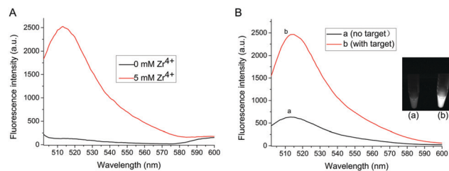
Fig. 1 (A) The fluorescence intensity in the presence of exosomes and liposomes corresponding to the Triton X-100 treated calcein-encapsulated liposomes before (dark line) and after adding \text{Zr}^{4+} (red line). (B) Fluorescence spectra and images (inset) corresponding to the Triton X-100 treated calcein-encapsulated liposomes after (a) incubated with PBS buffer and (b) incubated with exosomes. The concentration of exosomes is 2.1 \times 10^7 particles per \mu\text{L} .
