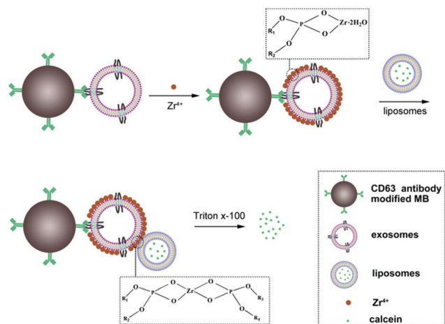
Scheme 1 Working principle of the assay for the detection of exosomes based on phosphate– \text{Zr}^{4+} coordination interaction and liposome-based signal amplification. In order to clearly display the exosome–zirconium–liposome sandwich structure, the diameter of MB, exosomes and liposomes doesn't represent real size contrast.
