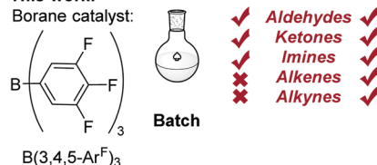
Fig. 1 Previous work on borane catalysed hydroboration with conventional conditions (top) and this work, assisted with enabling technologies (bottom).
