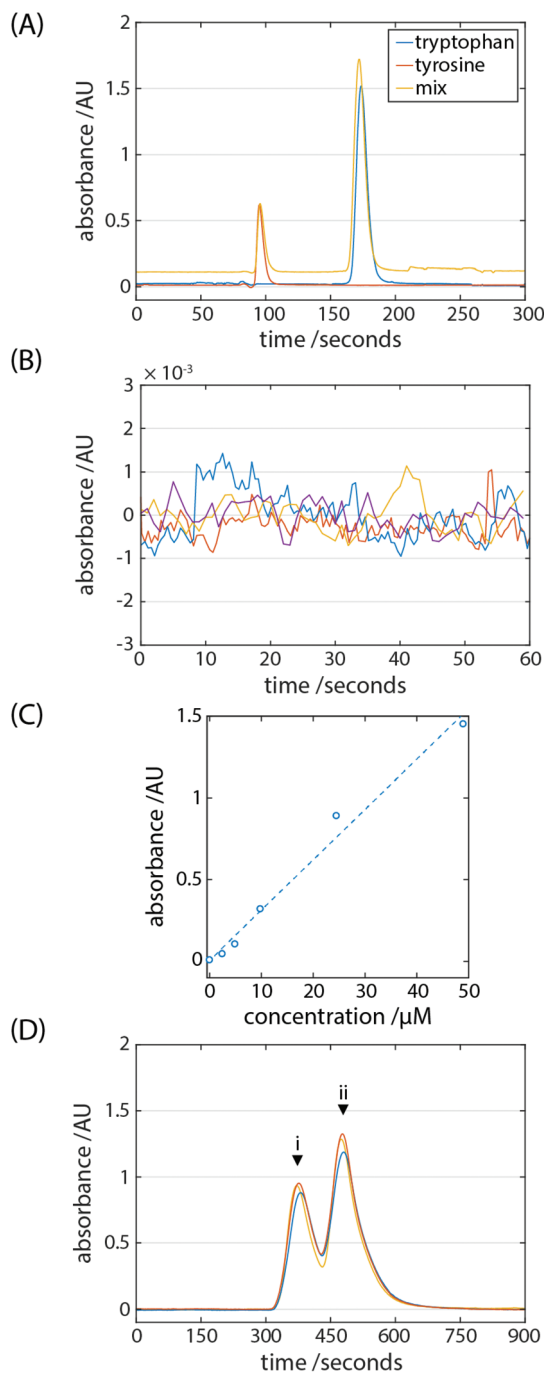
Fig. 3 Separations are performed on the system using the pressurised-gas pump. (A) A mix of the amino acids tryptophan and tyrosine are separated and identified using a UV-LED absorption detector arrangement. The mix trace is vertically shifted for clarity. (B) The baseline noise of the detector is shown. (C) A concentration series is established plotting peak heights for tryptophan spanning 2.4 \mu\text{M} ( 4.8 \text{ pmol} ) to 49.0 \mu\text{M} ( 98 \text{ pmol} ). The error bars lie within the points. (D) A mix of the pesticides (i) thiabendazole and (ii) pyrimethanil are separated.
