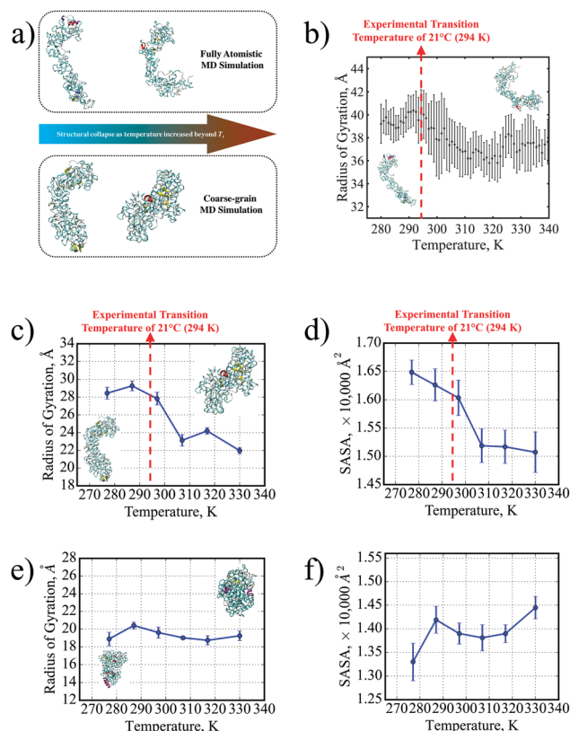
Fig. 2 (a) A distinct structural transition temperature for SE_{8Y} was captured by both FAMD and CGMD in terms of (b) the radius of gyration and (d) the SASA from CGMD. This is contrasted with the absence of distinct transitions in S_4E_{8Y} in terms of the (e) radius of gyration and (f) SASA as well. Insets in both (c) and (e) show the respective SELP molecule's conformations at 277 K (left) and 330 K (right).
