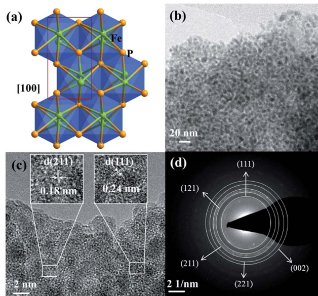
Fig. 6 (a) The crystal structure of \text{FeP} crystallizing in the orthorhombic space group Pna2_1 (shown along [100] ; the unit cell is shown in red). (b) TEM image displaying homogeneously distributed nanoparticles of 2–5 nm in size. (c), HR-TEM image with d -spacing of 0.18 and 0.24 nm (in the inset) corresponding to (211) and (111) planes. (d) SAED pattern exhibiting characteristic rings confirming the phase-purity of \text{FeP} (JCPDS 71-2262).
