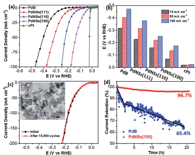
Fig. 5 Electrocatalytic HER performances of different PdNSs in 0.5 \text{ M H}_2\text{SO}_4 . (a) LSV curves of PdNSs \{100\} , PdNSs \{110\} , PdNSs \{111\} , PdB and cPt at a scan rate of 5 \text{ mV s}^{-1} . (b) Electrocatalytic HER activities of PdNSs \{100\} , PdNSs \{110\} , PdNSs \{111\} , PdB and cPt at current density of 10, 50 and 100 \text{ mA cm}^{-2} , respectively. (c) LSV curves of PdNSs \{100\} before and after repeating CV scans of 15 000 cycles at 50 \text{ mV s}^{-1} . Inserted in (c) is the TEM image of PdNSs \{100\} after test for 15 000 cycles. (d) Time-dependent i - t curves of PdNSs \{100\} and commercial PdB under a constant overpotential of 42 mV at 50 \text{ mA cm}^{-2} .
