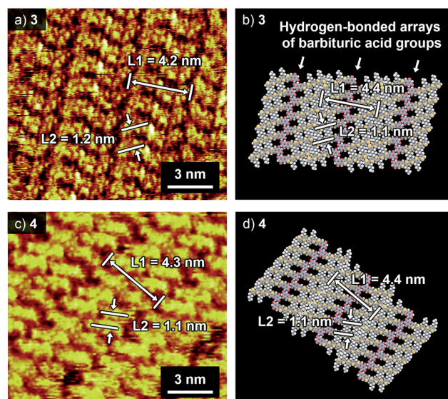
Fig. 2 (a and c) STM images of (a) 3 and (c) 4 at the 1-phenyloctane–HOPG interface. Tunneling current ( I_t ) = 9 pA, bias voltage ( V_s ) = +0.65 V. The concentration of the solution is 5 \times 10^{-6} M. (b and d) Molecular models of two-dimensionally arranged tapelike supramolecular polymers of (b) 3 and (d) 4 based on the STM images.
