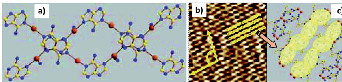
Fig. 24 (a) Double-stranded coordination helicate 2. (b) AFM image of 2 on HOPG surface. Image size is 400 \times 400 \text{ \AA}^2 ; (c) proposed model of adenine-silver helicate deposition. (Reproduced with permission from ref. 118 © 2007 American Chemical Society).
