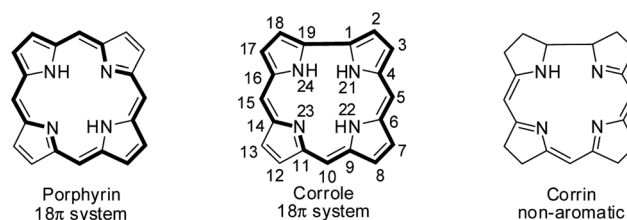
Fig. 1 Skeletal structure of porphyrin, corrole and corrin.
