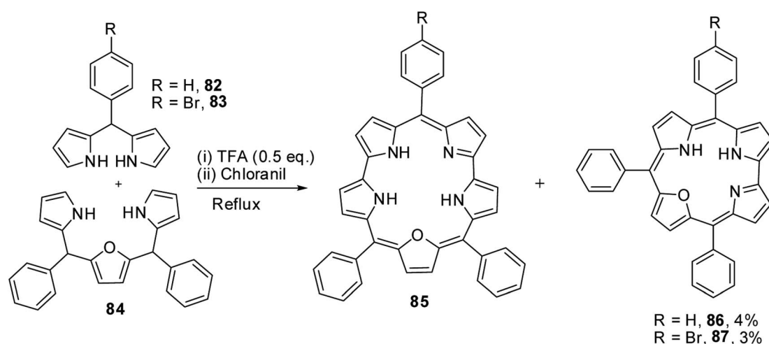
Scheme 21 Synthesis of meso -substituted 22-oxacorrroles 86 and 87 .
