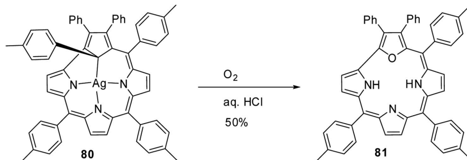
Scheme 20 Synthesis of 21-oxacorrrole 81 from Ag(III) carbacorrrole 80 .
