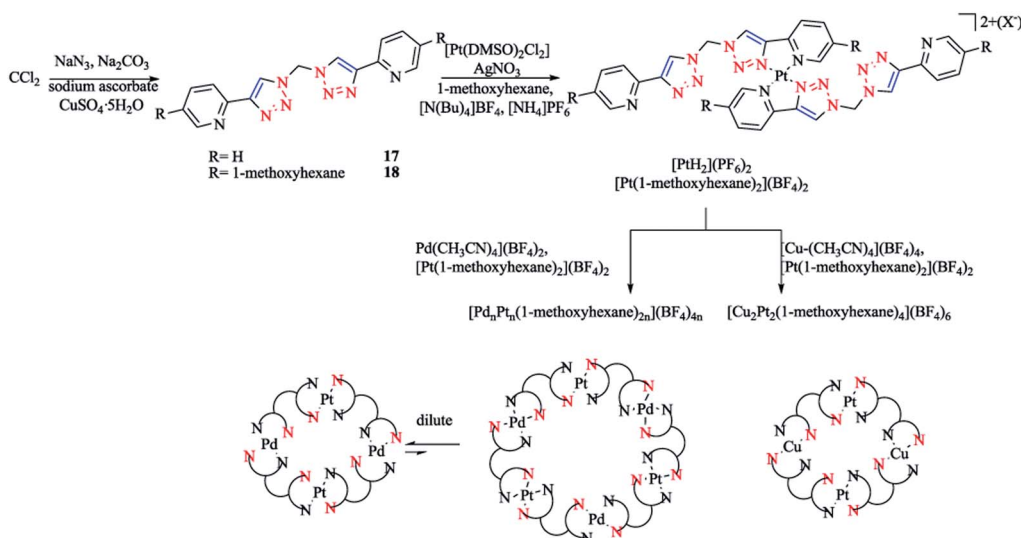
Scheme 12 Synthesis of heterometallic [\text{M}_n\text{Pt}_n(\text{L})_{2n}]^{x+} macrocycles based on dichloromethane-derivative bis-2-pyridyl-1,2,3-triazole ligands.
