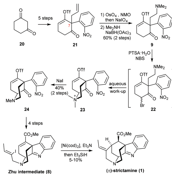
Scheme 4 Zhu's total synthesis of ( \pm )-strictamine.
