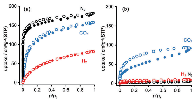
Fig. 8 Gas adsorption isotherms of (a) TpMe-apo and (b) TpF-apo for \text{CO}_2 (cyan) at 195 K, \text{H}_2 (red) at 77 K and \text{N}_2 (black) at 77 K. Solid and open symbols denote adsorption and desorption processes, respectively.
