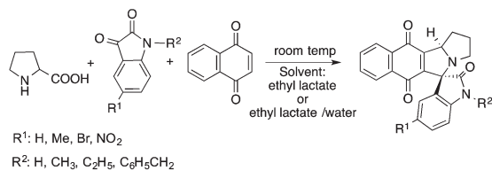
Scheme 24 Synthesis of spiro[benzo[ f ]pyrrolo[2,1- a ]isoindole-5,30-indoline]-20,6,11-trions.
