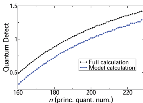
Fig. 4 Quantum defects for J = 0 HR states in the range n = 160\text{--}230 calculated using the full log derivative/MQDT approach outlined in the article, as well as a simple diabatic model (see text for details). The model calculations follow the trend for the full calculation closely.
