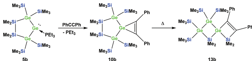
Scheme 8 Reaction of 5b with tolane gave the expected [4.2]-spirocyclic germacyclopropene 10b , which upon heating rearranged into the [3.3]-spirocyclic vinylgermane 13b .
