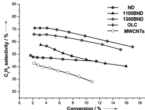
Fig. 7 Propylene selectivity versus propane conversion curves of UNDD catalysts with different annealing temperatures and MWCNTs in the ODH process. Reproduced from ref. 127 with permission Wiley, copyright 2014.
