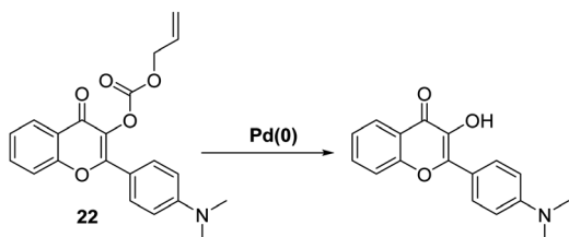
Scheme 21 \text{Pd} catalyzed decarboxylative deprotection of probe 22 , a process that allows for the ratiometric fluorescence detection of 0, +2 and +4 \text{Pd} species. Measurement conditions: PBS/THF (9 : 1) pH = 7.4.
