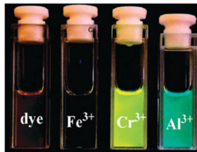
M = \text{Al}^{3+} ; \lambda_{\text{em}} = 527 \text{ nm} ; \phi_{\text{fl}} = 0.31 ; M = \text{Cr}^{3+} ; \lambda_{\text{em}} = 563 \text{ nm} ; \phi_{\text{fl}} = 0.63 ;
