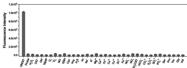
Fig. 1 Fluorescence response of TP-KA ( 1.0\ \mu\text{M} ) with various bio-analytes, including \text{ONOO}^- ( 10.0\ \mu\text{M} ), \text{H}_2\text{O}_2 ( 200\ \mu\text{M} ), other ROS and RNS ( 10.0\ \mu\text{M} ), GSH and Cys ( 5.0\ \text{mM} ), and other interfering substances ( 100\ \text{mM} ). The data were recorded after the incubation of TP-KA with various bioanalytes for 10 min at 37\ ^\circ\text{C} in PBS buffer ( 50\ \text{mM} , 7.4 ) with 1\% DMSO. The values are the mean \pm s.d. for n = 3 . \lambda_{\text{ex}}/\lambda_{\text{em}} = 430/560\ \text{nm} .
