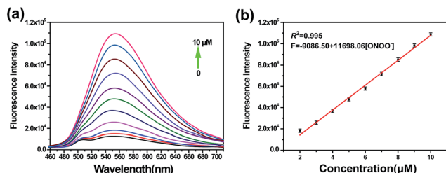
Fig. 2 (a) Fluorescence response of TP-KA ( 1\ \mu\text{M} ) to \text{ONOO}^- ( 0\text{--}10\ \mu\text{M} ) in PBS buffer ( 50\ \text{mM} , \text{pH}\ 7.4 ) with 1\% DMSO. (b) The linear curve derived from the fluorescence intensity at 560\ \text{nm} and the \text{ONOO}^- concentration. The spectra were recorded after the incubation of TP-KA with \text{ONOO}^- for 10 min at 37\ ^\circ\text{C} . The values are the mean \pm s.d. for n = 3 . \lambda_{\text{ex}}/\lambda_{\text{em}} = 430/560\ \text{nm} .
