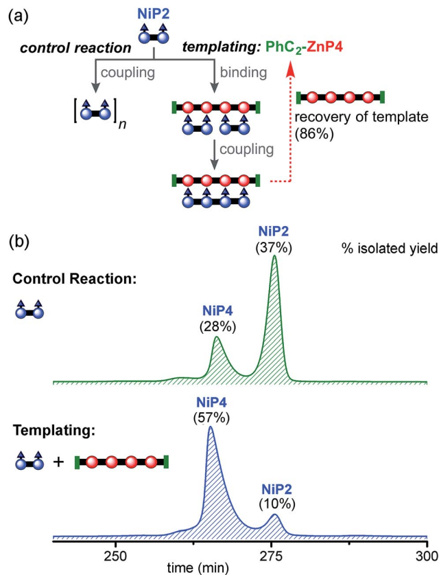
Fig. 7 Reaction design and outcome of linear tetramer templating for the synthesis of NiP 4 from NiP 2 , using PhC 2 -ZnP4 as the template. (a) Reaction scheme. (b) GPC traces (detection at 646 nm, toluene/1% pyridine) of the non-templated reaction (top) and the templated reaction (bottom) product mixture after removal of the template PhC 2 -ZnP4. The product NiP 4 and unreacted starting material NiP 2 were isolated and identified by MALDI-ToF MS and 1 H NMR spectroscopy.
