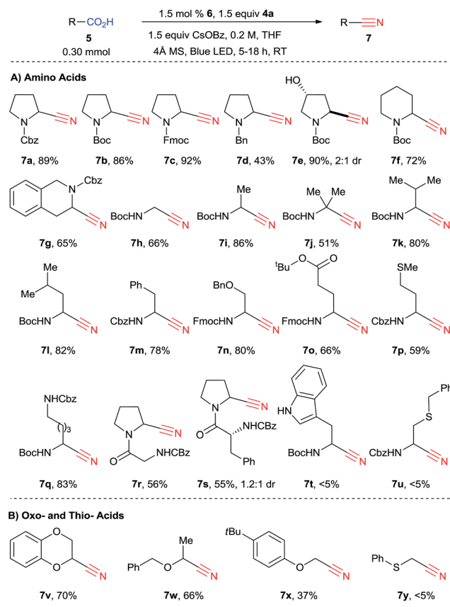
Scheme 4 Scope of carboxylic acids. Reaction conditions: carboxylic acid (5, 0.30 mmol, 1.0 equiv.), CBX reagent (4a, 0.45 mmol, 1.5 equiv.), 6 (4.5 \mu\text{mol} , 0.015 equiv.), CsOBz (0.45 mmol, 1.5 equiv.), 4 \text{\AA} molecular sieves (30 mg), THF (1.5 mL), 25–34 ^\circ\text{C} , blue LEDs irradiation for 5 to 18 h. Isolated yield after purification by column chromatography is given.
