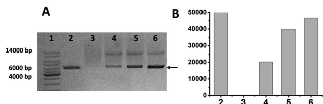
Fig. 1 The binding of pGal-sGFP and PGHNs was analyzed using agarose gel electrophoresis. (A) Lane 1, 1 kb DNA ladder; lane 2, pGal-sGFP DNA; lane 3, PGHNs; lane 4–6 represented PGHN–DNA mixture prepared with different volume ratios (the volume of PGHNs was 0, 100, 90, 60, and 30 \mu\text{L} , respectively, where DNA volume was always 10 \mu\text{L} except for lane 3 (0)). (B) The intensity of the lower DNA band (A: arrow) was quantified.
