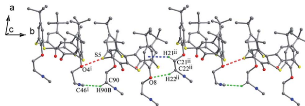
Fig. 20 A 1-D chain of 24 , showing the \text{C}\cdots\text{H}\cdots\text{C} (green), \text{C}\cdots\text{H}\cdots\text{O} (green), \text{C}\cdots\text{H}\cdots\pi (blue) and \text{O}\cdots\text{S} (red) interactions.
