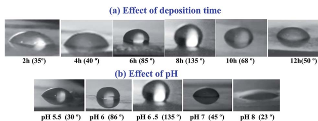
Fig. 15 Contact angle photographs for ZnO nanostructured films fabricated at different (a) deposition time and (b) pH value.
