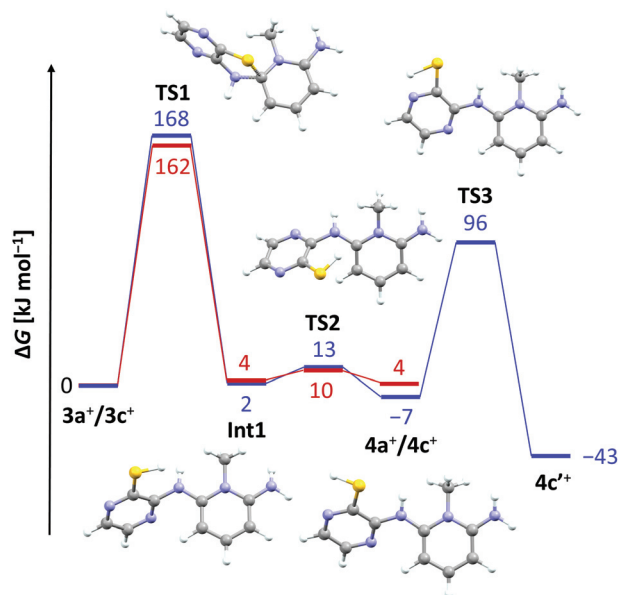
Fig. 2 Reaction coordinate diagram (PBE1PBE-IEFPCM/def2-TZVP) for the Smiles rearrangement reaction of 3a ^+ (red) and 3c ^+ (blue). For clarity, the structures of intermediates and transition states are only shown for the pathway from 3c ^+ to 4c ^{++} .
