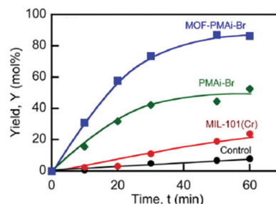
Fig. 17 5-HMF yield (%) from fructose at 100 °C. Conditions: DMSO, 5 mL; D-fructose concentration ( C f ), 0.555 mol L -1 ; catalyst loading, 50 mg mL -1 . Control: DMSO solvent with no catalysts added. Reprinted with permission from ref. 122. Copyright 2014, American Chemical Society.
