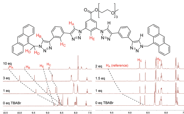
Fig. 2 Top: Labeling of protons monitored in ^1\text{H} NMR anion binding studies (consistent across 1–4 ). Bottom left: Partial ^1\text{H} NMR spectra of 2a titrated with TBABr. Bottom right: Partial ^1\text{H} NMR spectra of a competition experiment where 2b with 5 mol% of 2a as reference is titrated with TBABr (500 MHz, \text{CDCl}_3 , 298 K).
